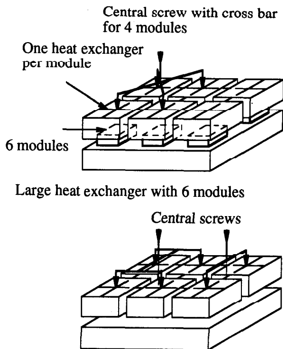
Figure 2. Tightening mechanisms
