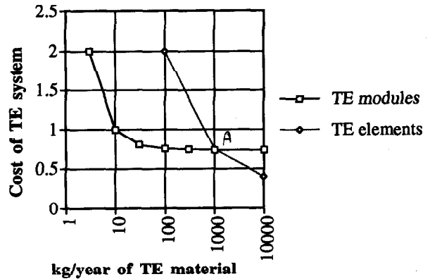
Fig. 6 Cost of TE system
