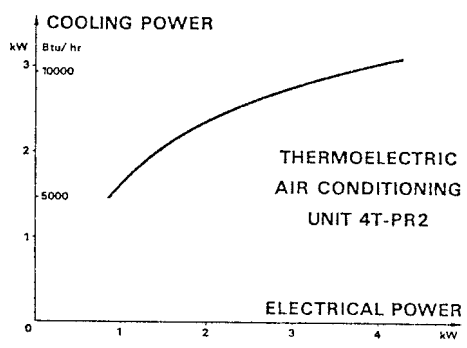
Fig.17. : COOLING POWER OF 4T PR2 UNIT
