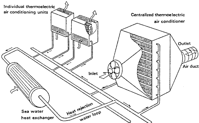
Fig.12. : SUBMARINE THERMOELECTRIC AIR CONDITIONING
