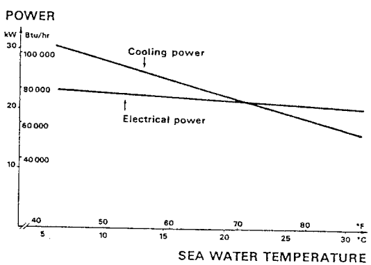
Fig.13. : PERFORMANCES OF AIR CONDITIONING CABINET 10T403
