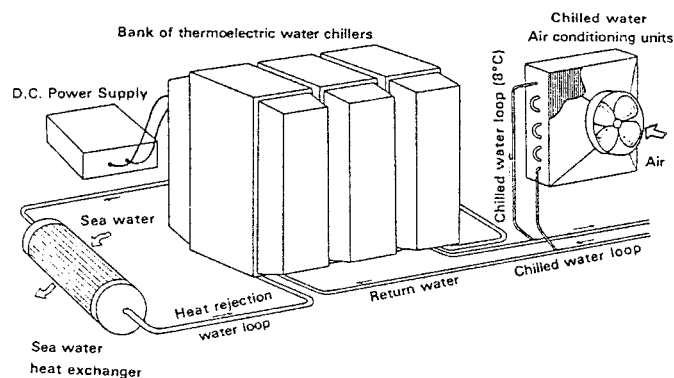
Fig.5. : SUBMARINE CENTRALIZED THERMOELECTRIC WATER CHILLER FOR AIR CONDITIONING
