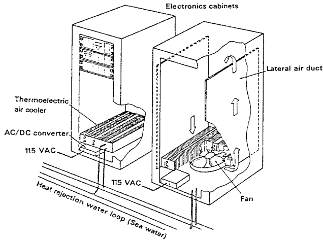
Fig.14. : THERMOELECTRIC AIR COOLING FOR ELECTRONIC CABINETS
