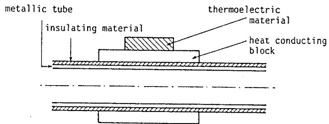
Fig.3. : CONTINUOUS TUBE WATER HEAT EXCHANGER
