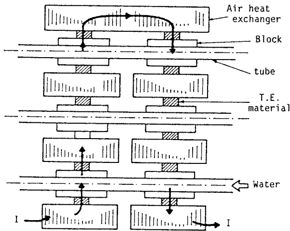
Fig.9. : SCHEMATIC OF WATER TO AIR THERMOELECTRIC ASSEMBLY
