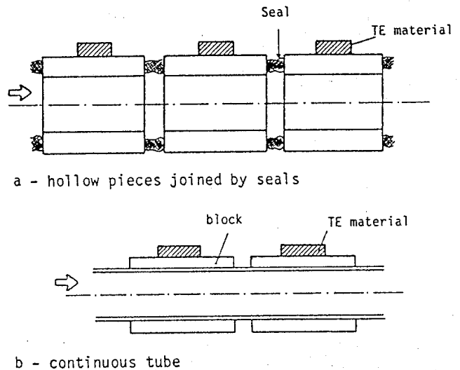
Fig.2. : SCHEMATICS OF WATER HEAT EXCHANGERS
