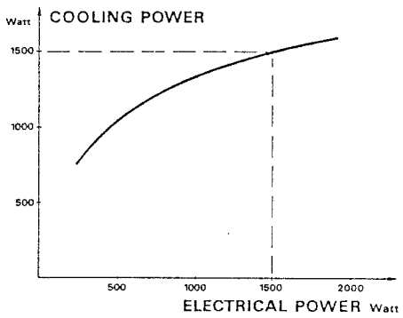
Fig.15. : COOLING POWER 19 INCHES RACK-UNIT EA 540
