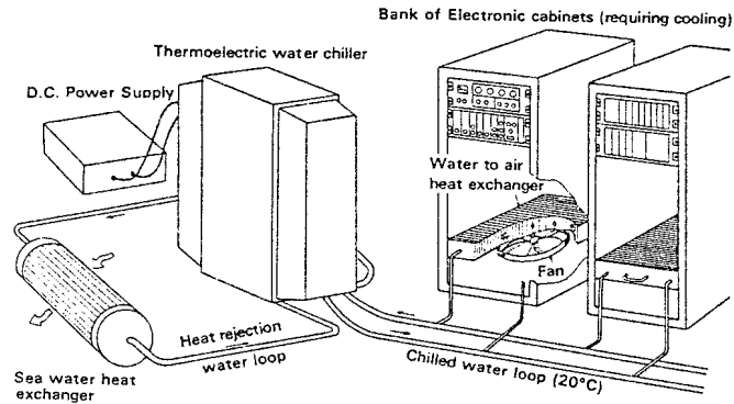
Fig.7. : SUBMARINE CENTRALIZED THERMOELECTRIC WATER CHILLER TO COOL ELECTRONIC CABINETS
