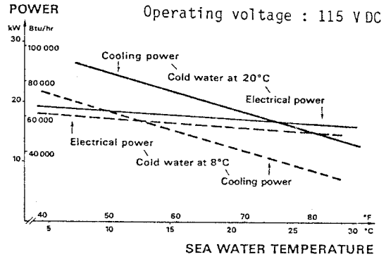
Fig.8. : THERMOELECTRIC WATER CHILLER 10T925 PERFORMANCES
